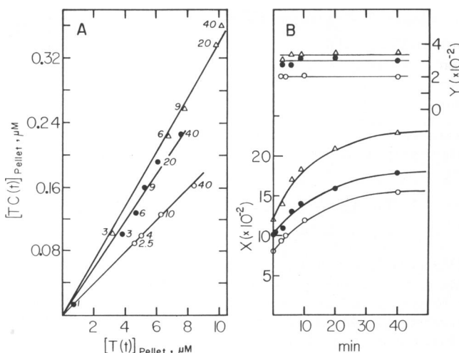
FIGURE 2 TC mole fractions in the polymer and solution phases during assembly. Microtubule protein preparations ( T_{\text{total}} \sim 14.5 \mu M ) were assembled at 37^\circ C in the presence of 1.2\text{-}\mu M ( \circ ), 1.6\text{-}\mu M ( \bullet ), and 2\text{-}\mu M ( \Delta ) (^3H)TC . Numbers adjacent to the data points in A indicate the time (minutes) after the start of assembly when 50\text{-}\mu M colchicine was added to abruptly arrest assembly (Materials and Methods). (A) Copolymer TC concentration vs. copolymer tubulin concentrations. Y during assembly, estimated from the slopes, had values of 1.9 \pm 0.2 \times 10^{-2} , 3.0 \pm 0.3 \times 10^{-2} , and 3.3 \pm 0.3 \times 10^{-2} for [TC]_{\text{total}} of 1.2, 1.7, and 2.0 \mu M , respectively. (B) TC mole fractions in the copolymer and solution phases, Y(t) and X(t) , respectively, plotted against time. Y(t) was obtained from the data displayed in A while X(t) was calculated from a material balance based on Y(t) values (Materials and Methods).
